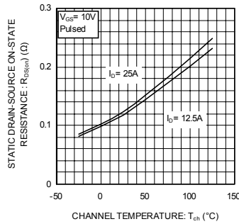
Fig.8 Static Drain-Source On-State Resistance vs. Channel Temperature
