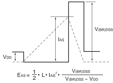
Fig.3-2 Avalanche waveform
