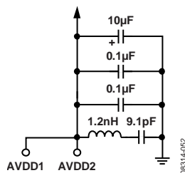
Figure 56. GSM Filter on the Analog Supply Pins
