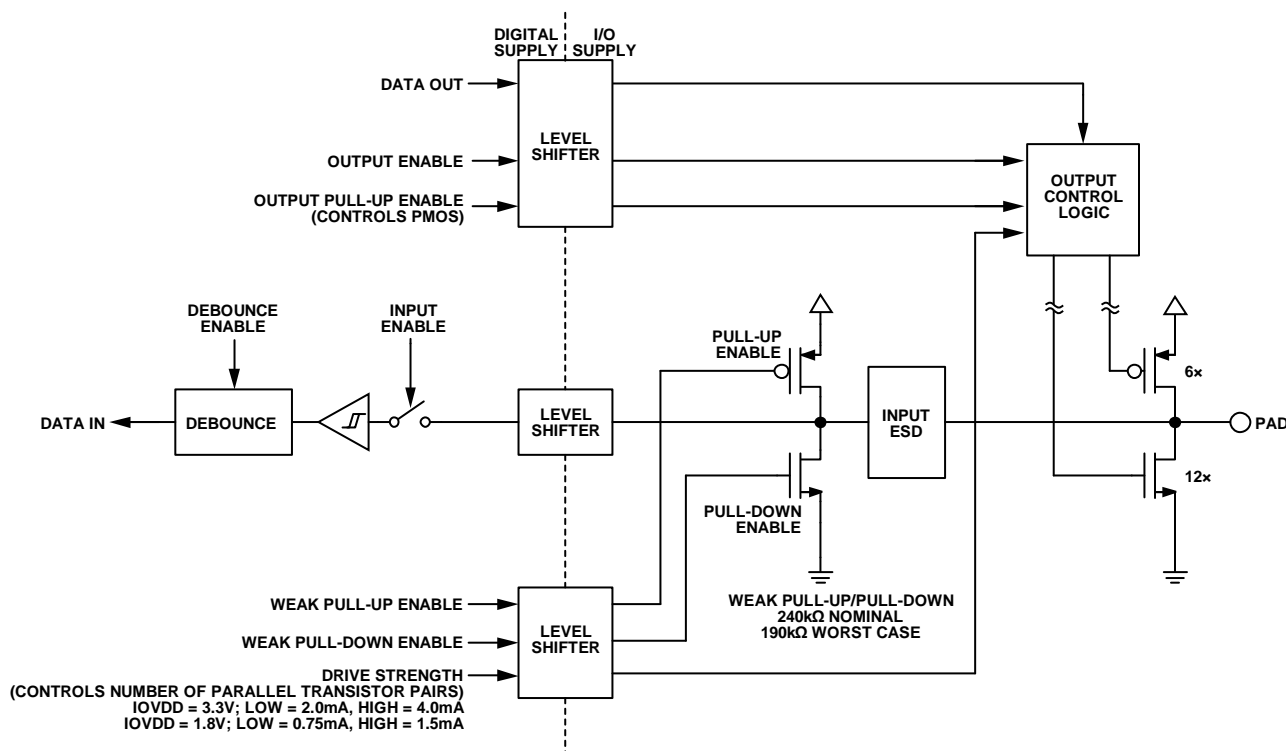
Figure 73. Pad Configuration, Internal Design
