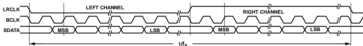
Figure 46. PS Mode—16 Bits to 24 Bits per Channel
