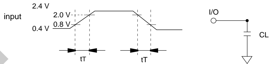
Input waveform and Output load
