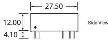
CTDD2710SF-D1K-1 Package
