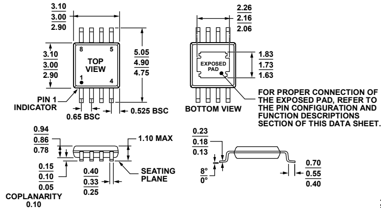
Figure 43. 8-Lead Mini Small Outline Package with Exposed Pad [MINI_SO_EP] (RH-8-1) Dimensions shown in millimeters
