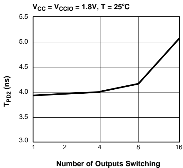
Figure 2: Derating Curve for T_{PD2}
