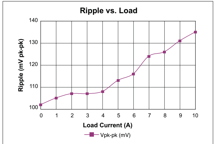
Figure 6 – V_{ripple} vs. I_{OUT} ; 48 V_{IN} ; no external output capacitance
