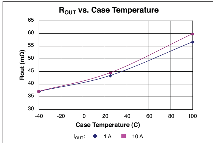
Figure 4 – R_{OUT} vs. temperature vs. I_{OUT}
