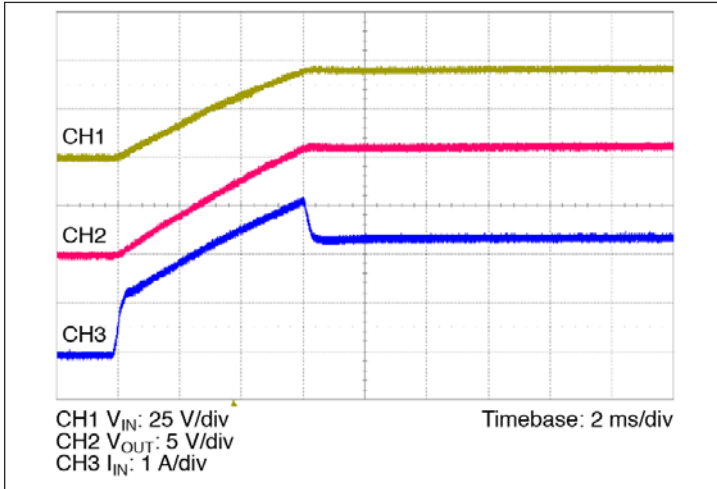
Figure 11 – Start up from application of V_{IN} ; VC pre-applied C_{OUT} = 500 \mu F
