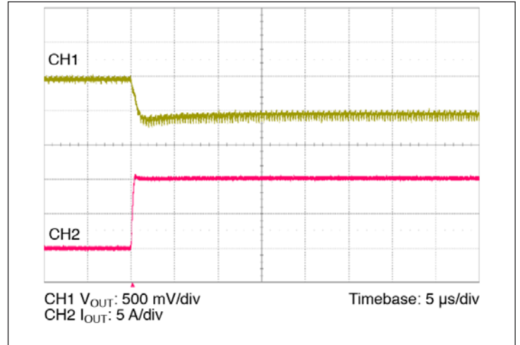
Figure 12 – 0 – 10 A transient response; C_{IN} = 100 \mu F , no external C_{OUT}
