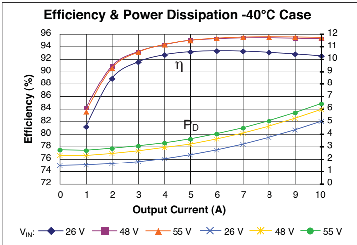
Figure 3a – Efficiency and power dissipation at -40°C (case); V_{IN}
