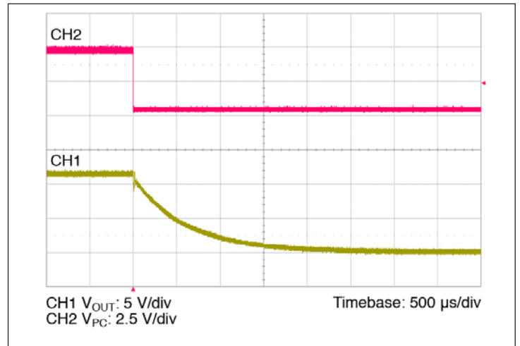
Figure 14 – PC disable waveform; R_{LOAD} = 1.2 \Omega , C_{OUT} = 500 \mu F
