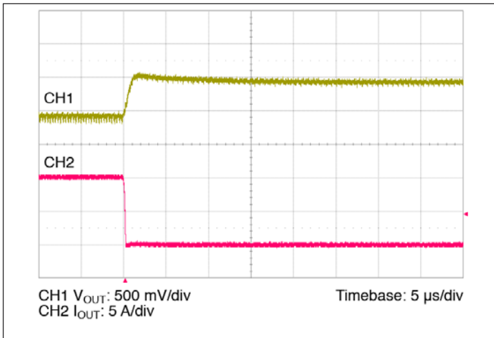
Figure 13 – 10 A – 0 A transient response; C_{IN} = 100 \mu F , no external C_{OUT}
