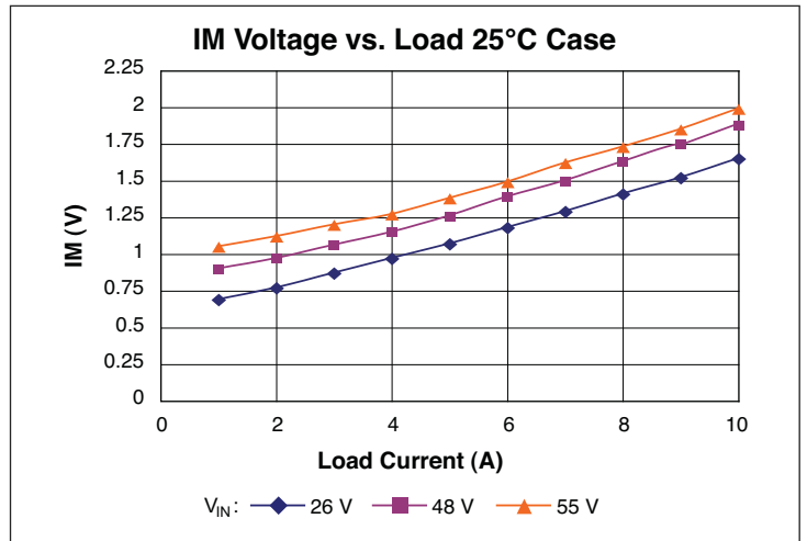
Figure 8 – IM voltage vs. load; 25°C Case
