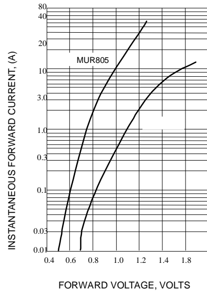
Fig. 5-TYPICAL FORWARD CURRENT
