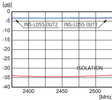
Transmission
