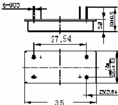
Package Outline
