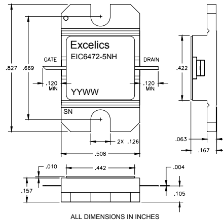
EIC6472-5NH (Non-Hermetic)
