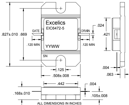
EIC6472-5 (Hermetic)
