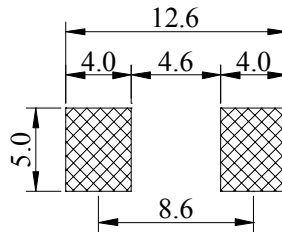
( PCB Pattern )
