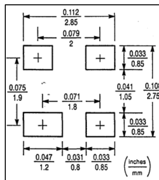
PAD LAYOUT
