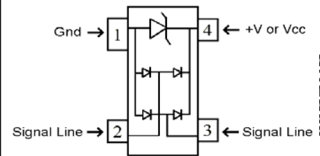
SCHEMATIC
