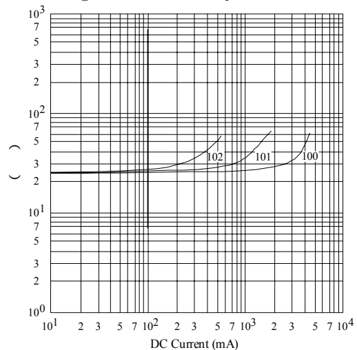
@ DC Current VS. Temp. Rise Curve
