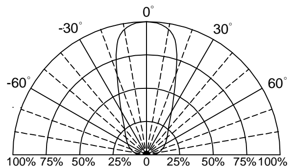
Directivity Radiation
