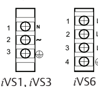
Figure 1. AC Input
