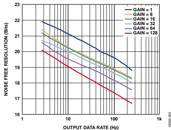
Figure 20. Noise-Free Resolution in Fast Settling Mode ( V_{\text{REF}} = 5 \text{ V} , Averaging by 16, \text{Sinc}^4 Filter, Chop Disabled)
