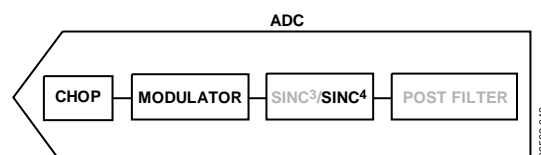
Figure 43. Chop Enabled
