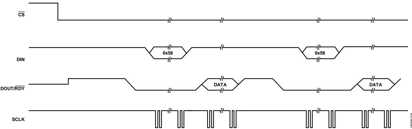
Figure 25. Continuous Conversion
