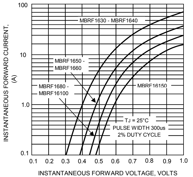
FIG.4-TYPICAL FORWARD CHARACTERISTICS
