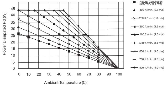
Power Dissipated vs Ambient Temperature And Air Flow - IFH200S
