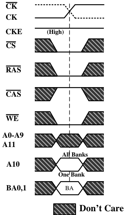
Figure 32. Precharge Command
