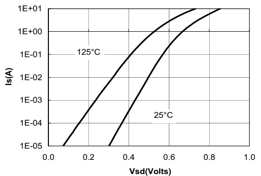
Figure 6: Body-Diode Characteristics
