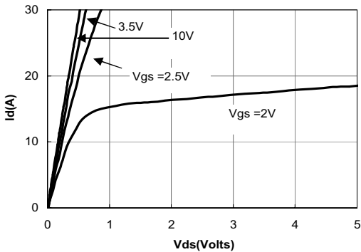
Figure 1: On-Regions Characteristics
