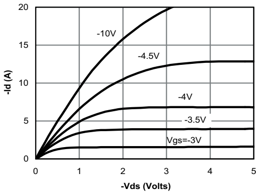
Fig 1: On-Region Characteristics
