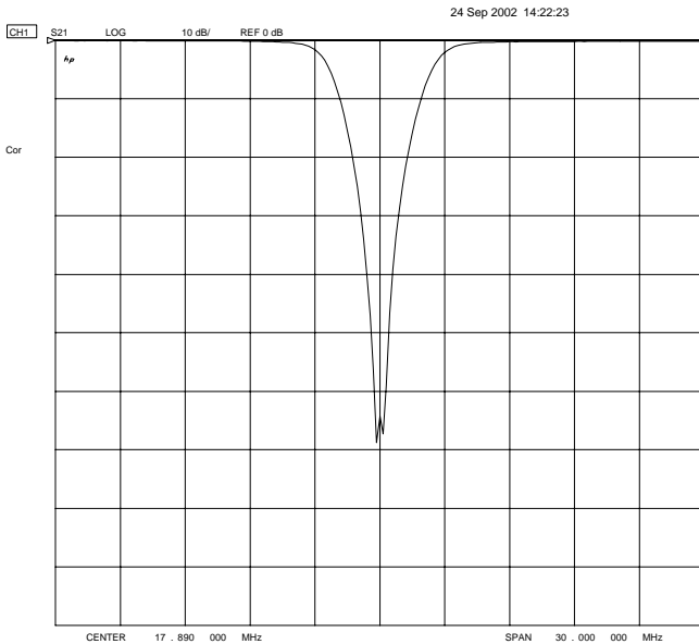
Amplitude Response (10 dB/div)
