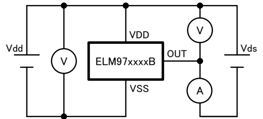
3)-(2) Output current (P-ch)
