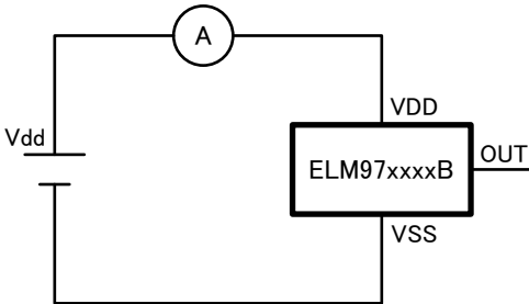
1) Current consumption
