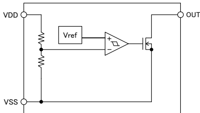
N-ch Output
