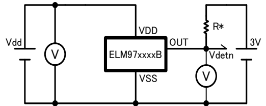
2) Detection voltage
