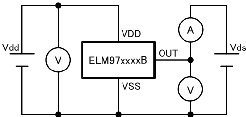
3)-(1) Output current (N-ch)
