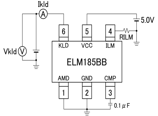
Ikld constant current test circuit
