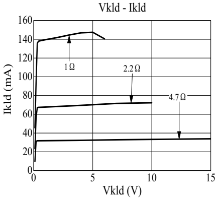
KLD output current voltage characteristics
