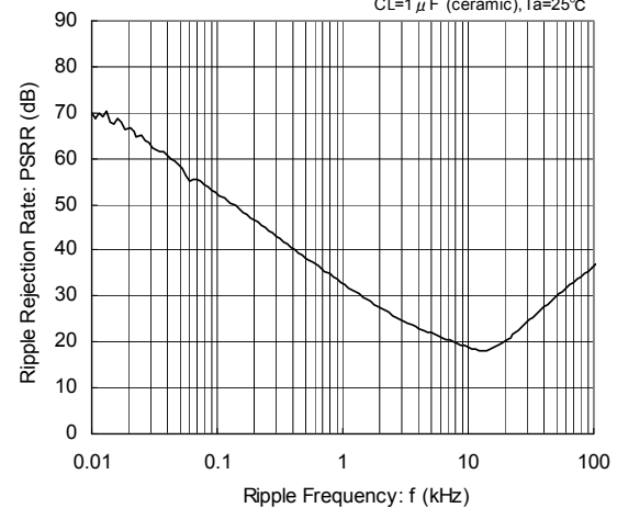
XC6216B/D 502
