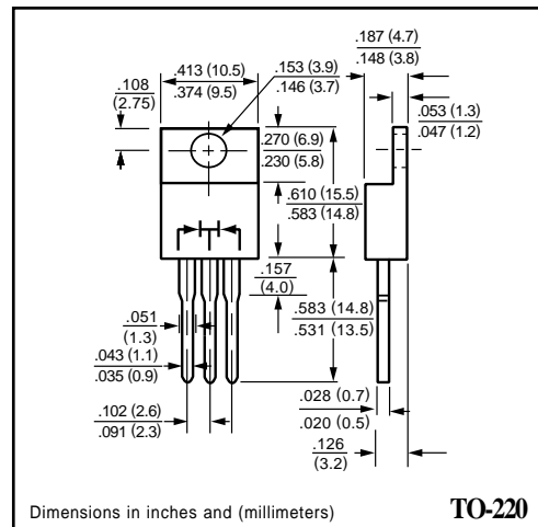
TO-220
