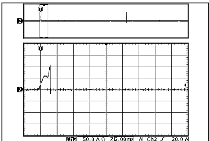
Figure 18: Load current ( 50\ \text{A}/\text{div} ) as a function of time when the converter attempts to turn on into a 1\ \text{m}\Omega short circuit. Bottom trace ( 2\ \text{ms}/\text{div} ) is an expansion of the on-time portion of the top trace.
