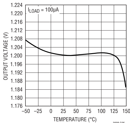
Output Voltage LT3008-1.2
