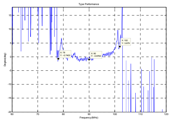
Phase Linearity(f0±12MHz)
