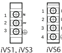
Figure 1. AC Input
