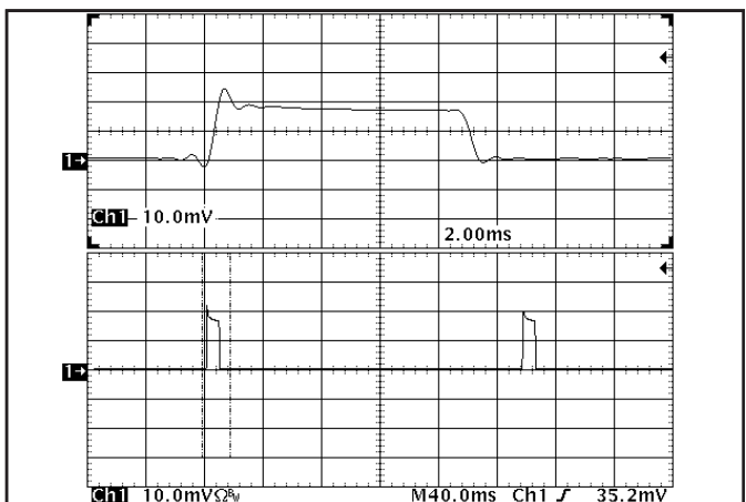
Figure 18: Load current ( 5\text{A}/\text{div} ) as a function of time when the converter attempts to turn on into a 10\ \text{m}\Omega short circuit. Top trace ( 2.0\text{ms}/\text{div} ) is an expansion of the on-time portion of the bottom trace.
