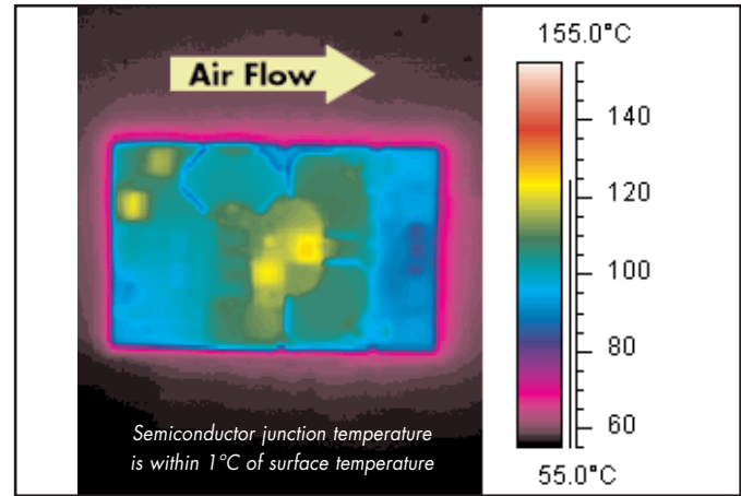
Figure 8: Thermal plot of converter at 6.0 amp load current (108W) with 55°C air flowing at the rate of 200 LFM. Air is flowing across the converter from input to output (nominal input voltage).
