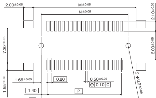
Recommended P.C.B. layout (View from mounting side)
