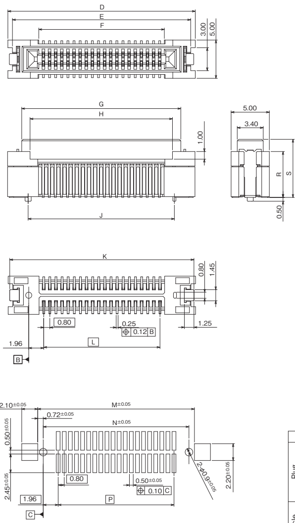
Recommended P.C.B layout (View from mounting side)
