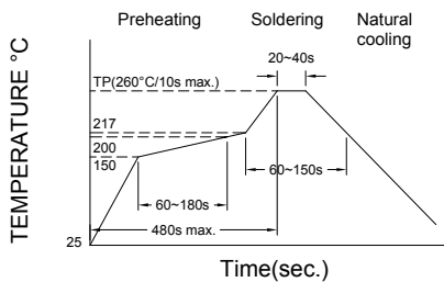
Figure 1. Re-flow Soldering
