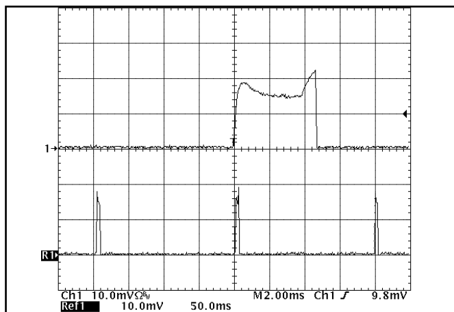
Figure 18: Load current ( 50\ \text{A}/\text{div} ) as a function of time when the converter attempts to turn on into a 1\ \text{m}\Omega short circuit. Top trace ( 2\ \text{ms}/\text{div} ) is an expansion of the on-time portion of the bottom trace.
