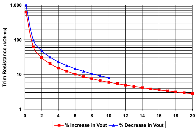
Figure C: Trim Graph for 2.0V out module
