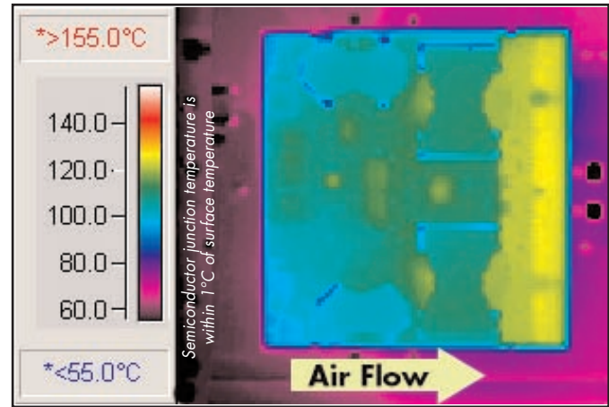
Figure 8: Thermal plot of converter at 49 amp load current with 55°C air flowing at the rate of 200 LFM. Air is flowing across the converter from input to output (nominal input voltage).
