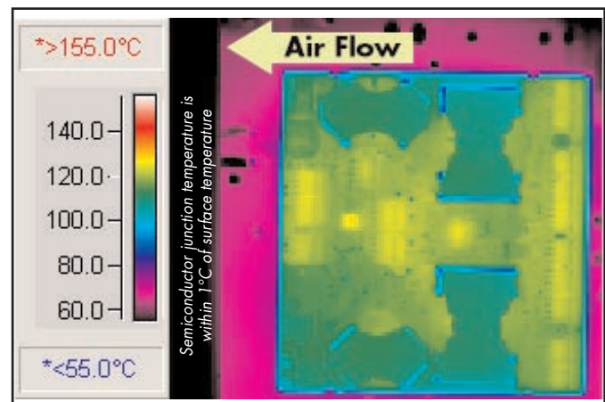
Figure 6: Thermal plot of converter at 53 amp load current with 55°C air flowing at the rate of 200 LFM. Air is flowing across the converter from output to input (nominal input voltage).
