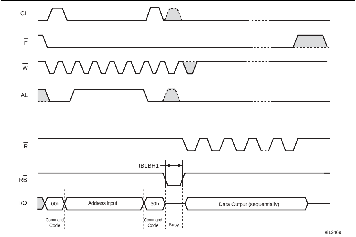
Figure 6. Read operations
