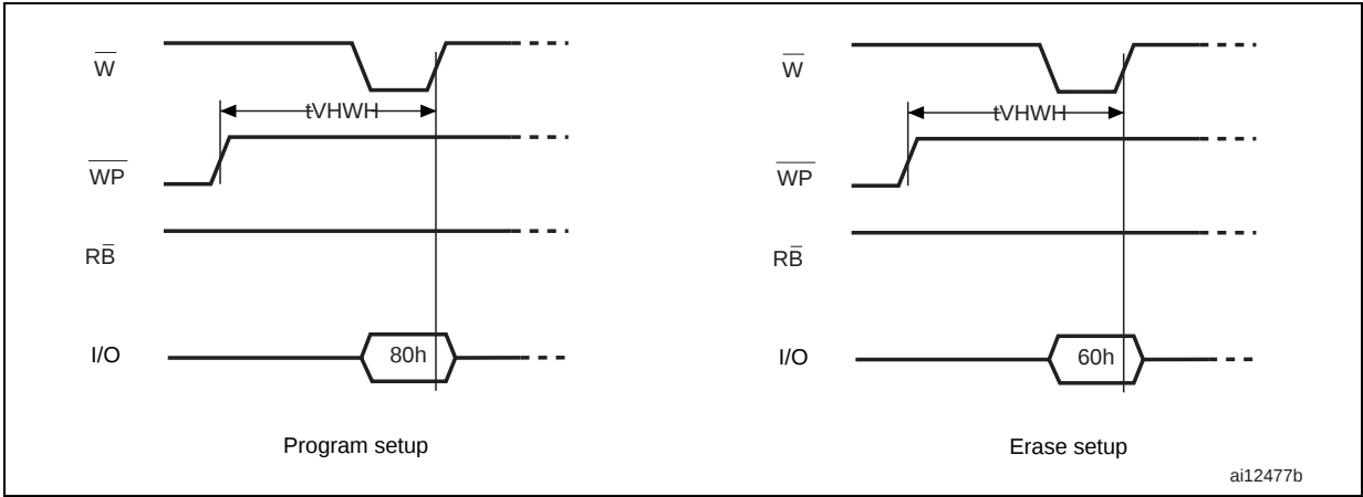
Figure 37. Program/erase enable waveform
