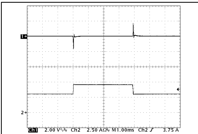
Figure 5: Output voltage response to step-change in load current (50%-75%-50% of I out (max); dI/dt = 0.08 A/μs). Load cap: 1 μF ceramic capacitor. Ch 1: V out (2 V/div), Ch 2: I out (2.5 A/div).
