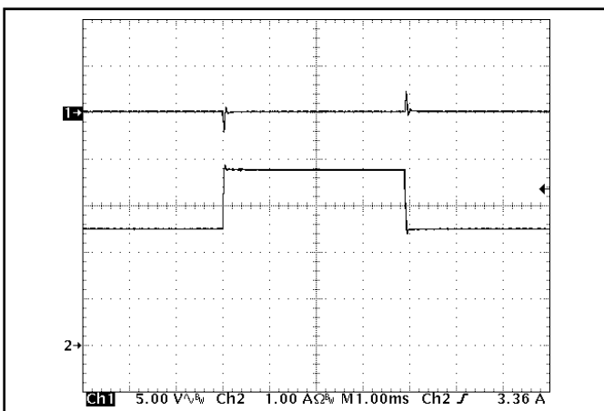
Figure 5: Output voltage response to step-change in load current (50%-75%-50% of I out (max); dI/dt = 0.05 A/μs). Load cap: 1 μF ceramic capacitor. Ch 1: V out (5 V/div), Ch 2: I out (1 A/div).
