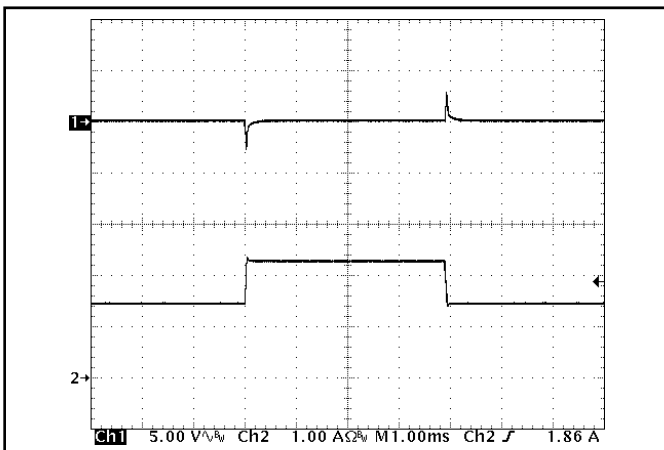
Figure 5: Output voltage response to step-change in load current (50%-75%-50% of I out (max); dl/dt = 0.02 A/μs). Load cap: 1 μF ceramic capacitor. Ch 1: V out (5 V/div), Ch 2: I out (1 A/div).
