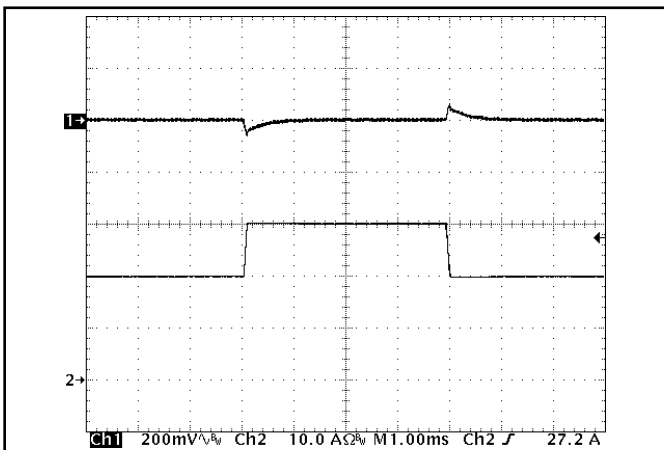
Figure 5: Output voltage response to step-change in load current (50%-75%-50% of Iout(max); dl/dt = 0.2 A/us). Load cap: 1 μF ceramic and 15 μF tantalum capacitors. Ch 1: Vout (200 mV/div), Ch 2: Iout (10 A/div).
