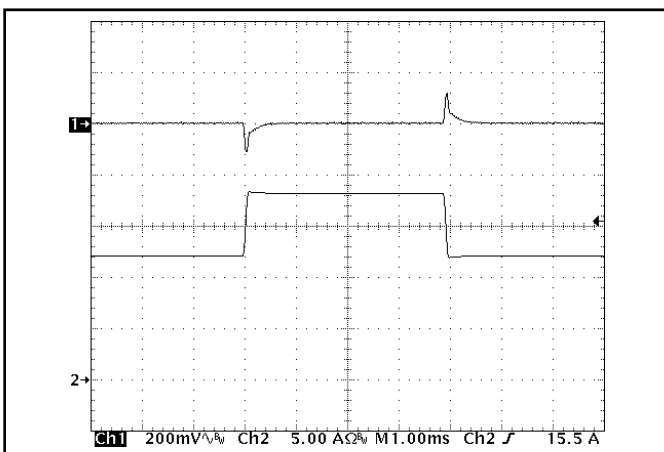
Figure 5: Output voltage response to step-change in load current (50%-75%-50% of I out (max); dl/dt = 0.1 A/us). Load cap: 1 μF ceramic and 15 μF tantalum capacitors. Ch 1: V out (200 mV/div), Ch 2: I out (5 A/div).
