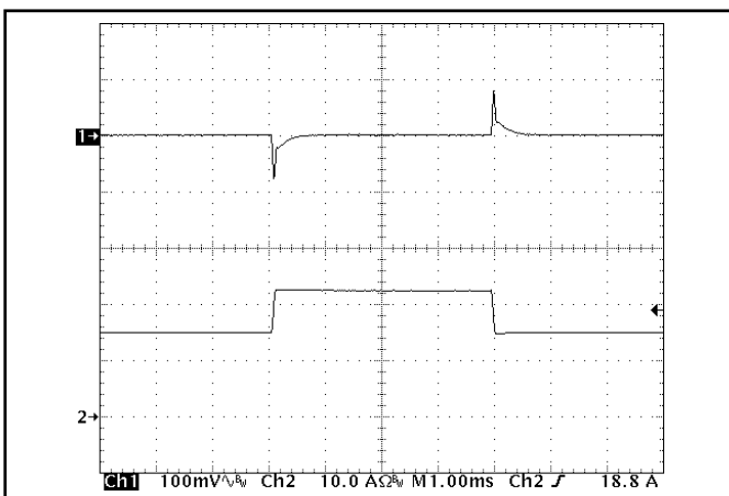
Figure 5: Output voltage response to step-change in load current (50%-75%-50% of Iout(max); dI/dt = 0.2 A/ \mu s). Load cap: 1 \mu F ceramic and 15 \mu F tantalum capacitors. Ch 1: Vout (100 mV/div), Ch 2: Iout (10 A/div).
