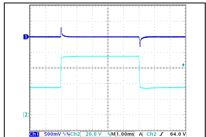
Figure 6: Output voltage response to step-change in input voltage (250 V/ms). Load cap: 100 \mu\text{F} , electrolytic output capacitance. Ch 1: V out (500 mV/div), Ch 2: V in (20 V/div).
