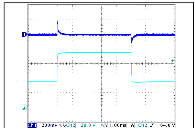
Figure 6: Output voltage response to step-change in input voltage (250 V/ms). Load cap: 100 \mu F, electrolytic output capacitance. Ch 1: Vout (200 mV/div), Ch 2: Vin (20 V/div).
