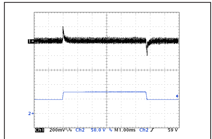
Figure 6: Output voltage response to step-change in input voltage (1000 V/ms). Load cap: 100 \mu F, electrolytic output capacitance. Ch 1: Vout (200 mV/div), Ch 2: Vin (50 V/div).
