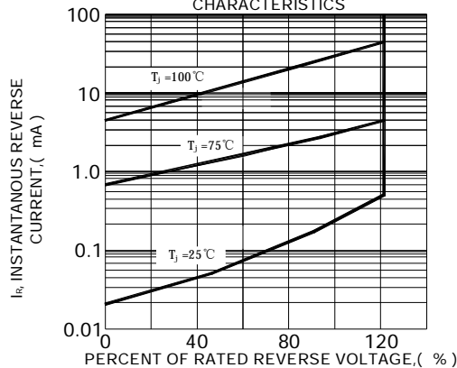
FIG.5-TYPICAL REVERSE CHARACTERISTICS
