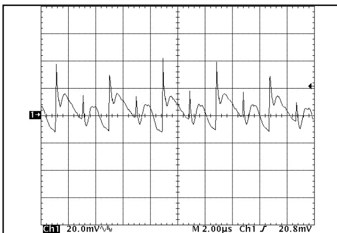
Figure 16: Output voltage ripple at nominal input voltage and rated load current (20 mV/div). Load capacitance: 1\ \mu\text{F} ceramic capacitor and 10\ \mu\text{F} tantalum capacitor. Bandwidth: 20 MHz. See Figure 13.
