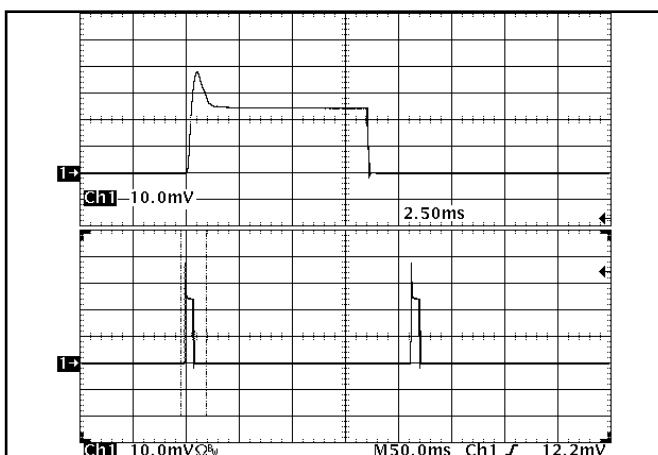
Figure 18: Load current (10A/div) as a function of time when the converter attempts to turn on into a 10\ \text{m}\Omega short circuit. Top trace (2.5ms/div) is an expansion of the on-time portion of the bottom trace.
