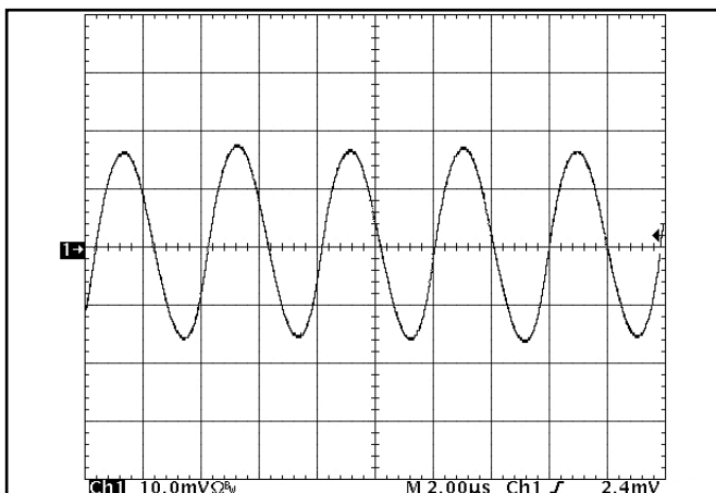
Figure 14: Input Terminal Ripple Current, i_c , at full rated output current and nominal input voltage with 10\ \mu\text{H} source impedance and 47\ \mu\text{F} electrolytic capacitor (100 mA/div). See Figure 13.
