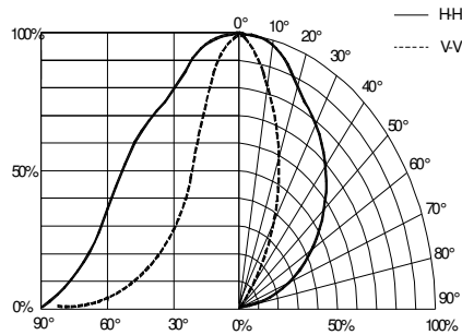
Relative Luminous Intensity vs. Radiation Angle
