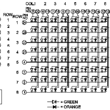
BL-M15A882XX
