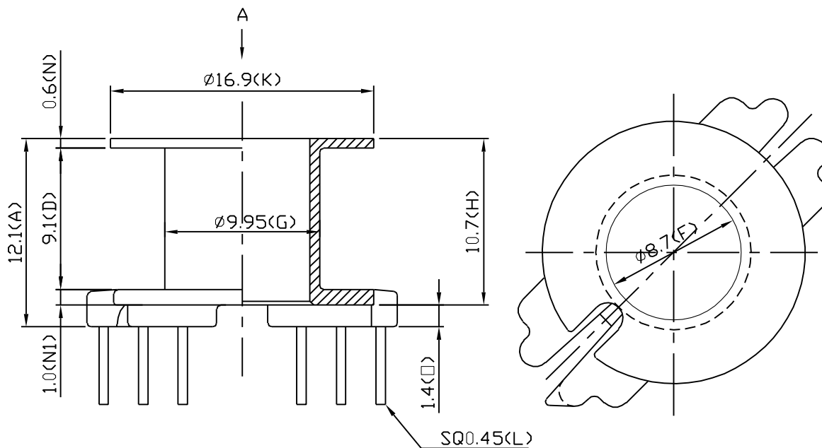
VIEW A
