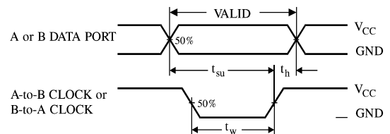
Figure 7. Switching Waveforms
