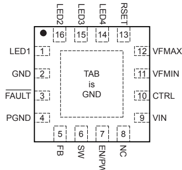
TQFN 16-Lead (Top View)
