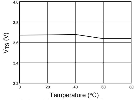
Fig.9 V TS (Low Temp) Limit vs. Temperature
