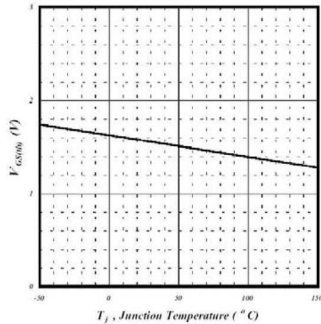
Fig 6. Gate Threshold Voltage vs. Junction Temperature
