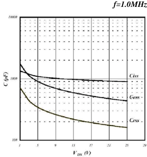
Fig 8. Typical Capacitance Characteristics
