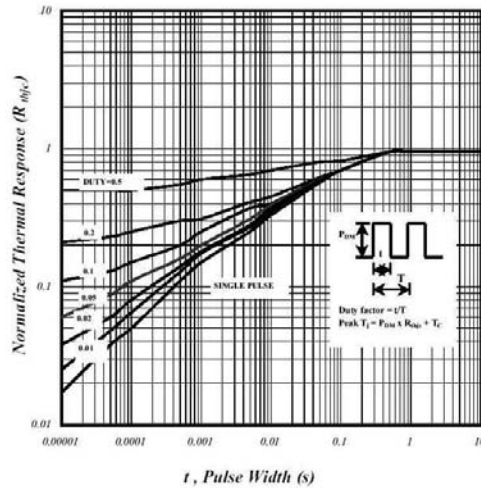
Fig 10. Effective Transient Thermal Impedance
