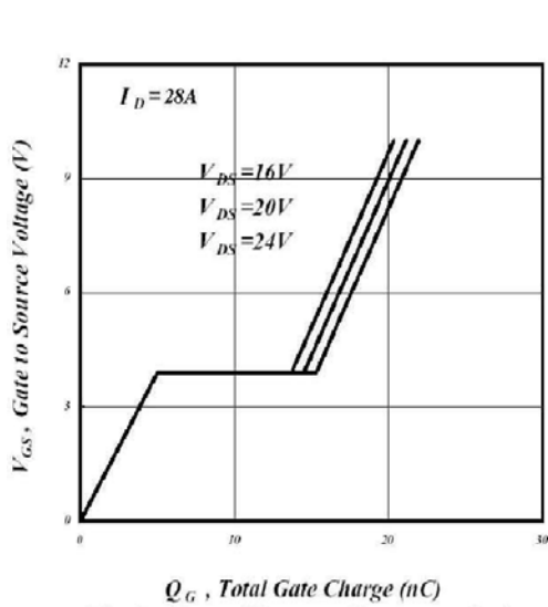
Fig 7. Gate Charge Characteristics
