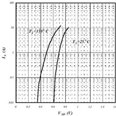
Fig 5. Forward Characteristics of Reverse Diode
